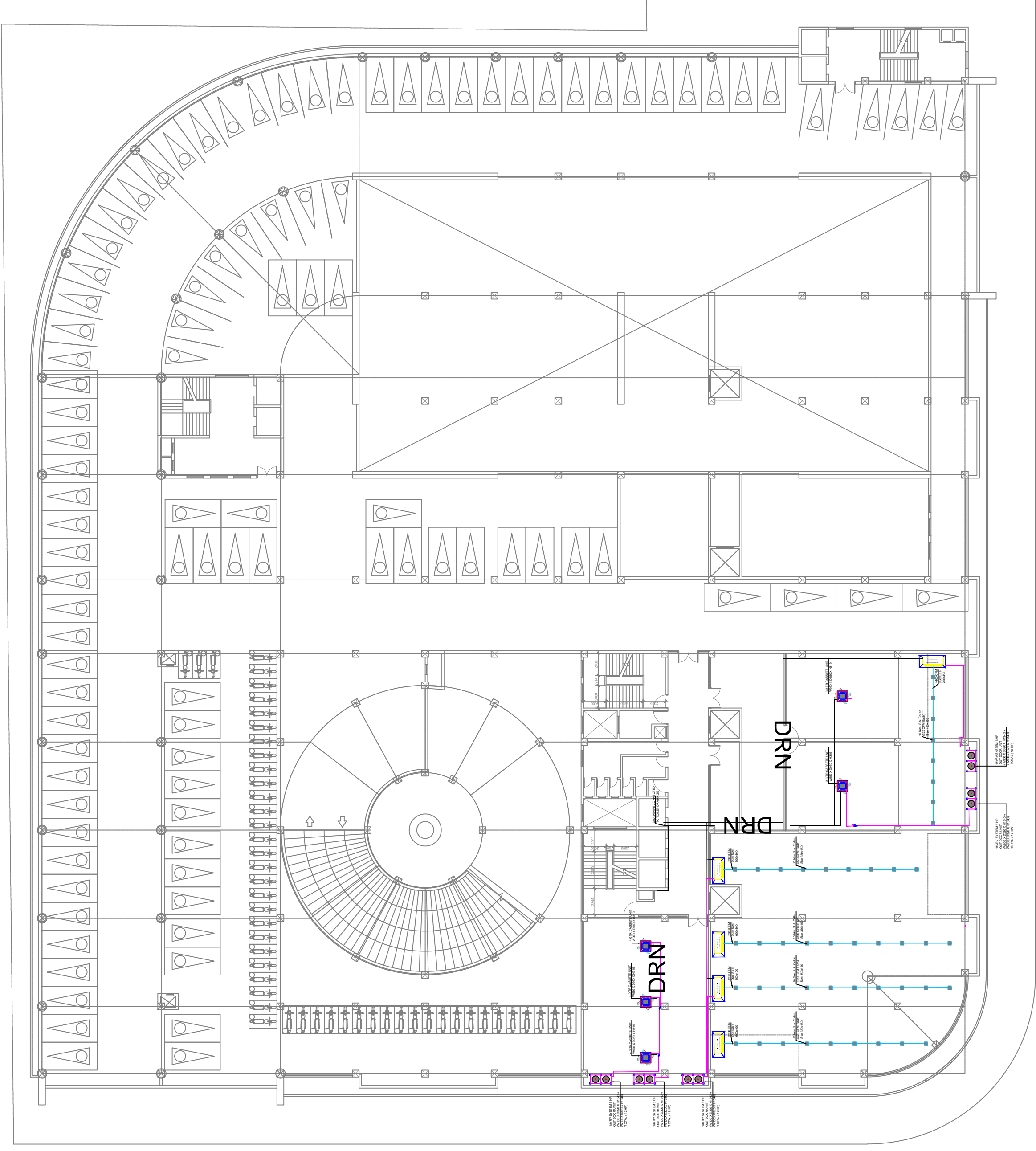
THIRD FLOOR PLAN +12.75 M LVL
