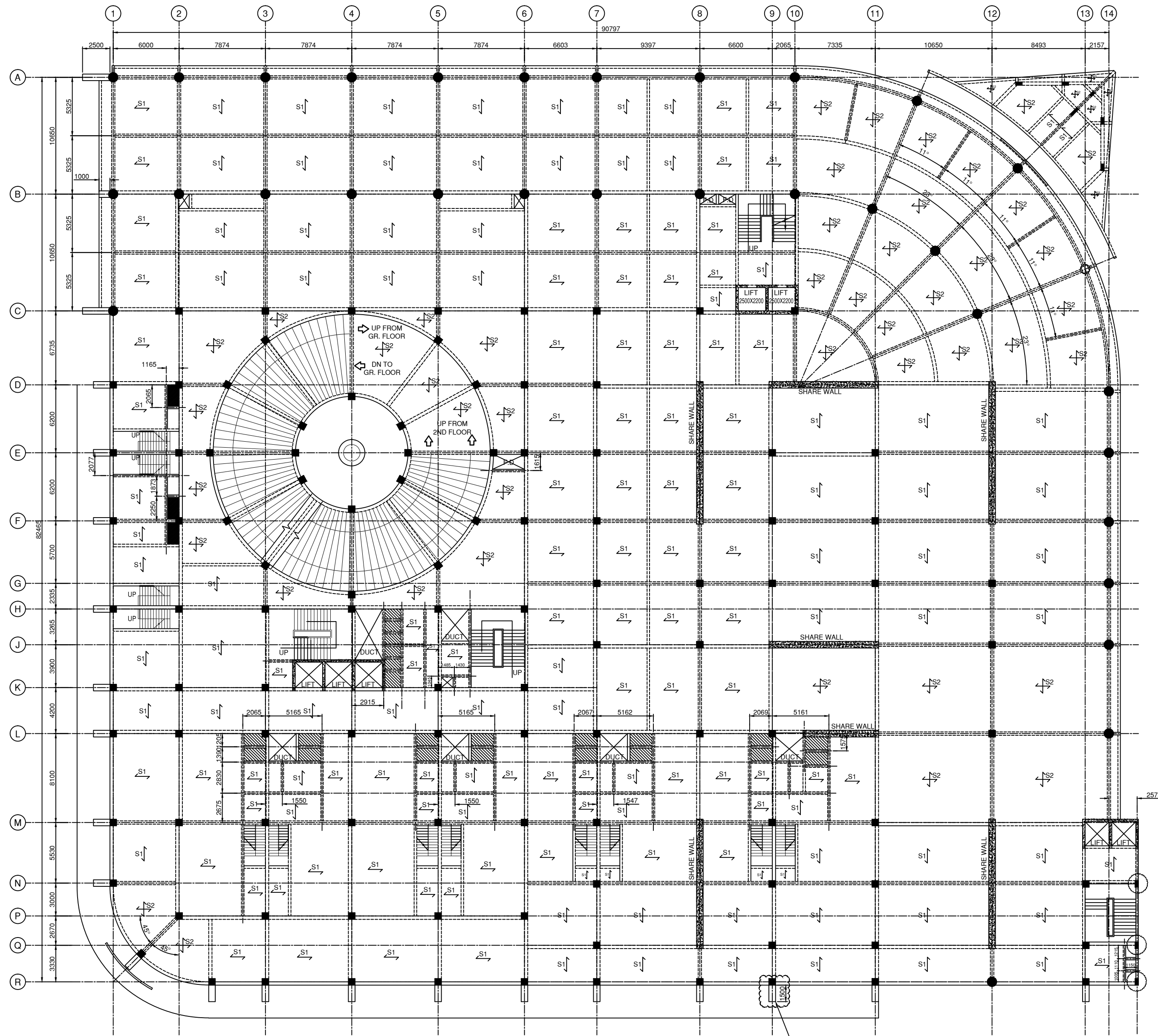
LAYOUT AT FIRST FLOOR EL(+4.80M LEVEL) SCALE 1:200
