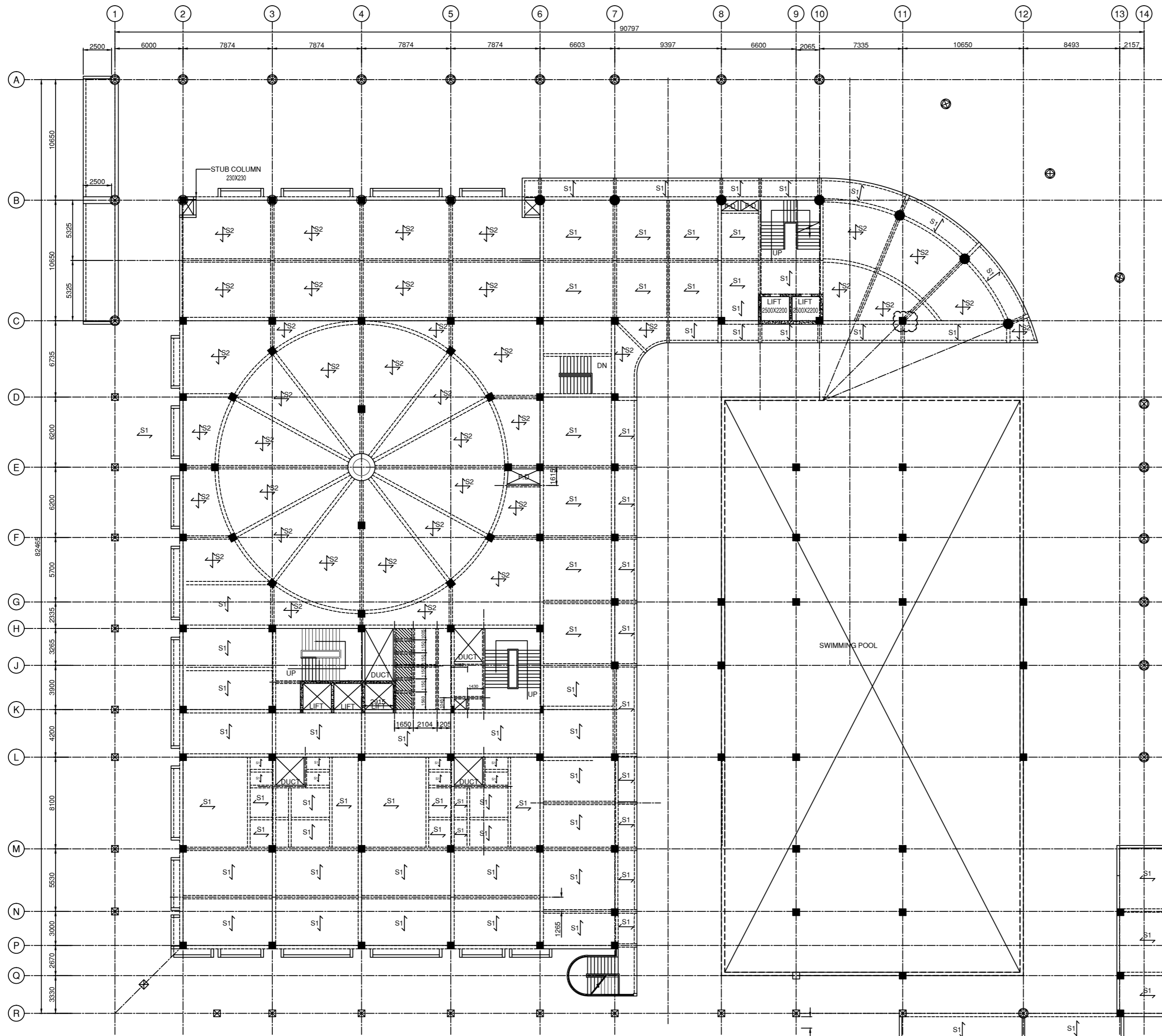
LAYOUT AT 5TH FLOOR EL(+19.20M LEVEL) SCALE 1:200
